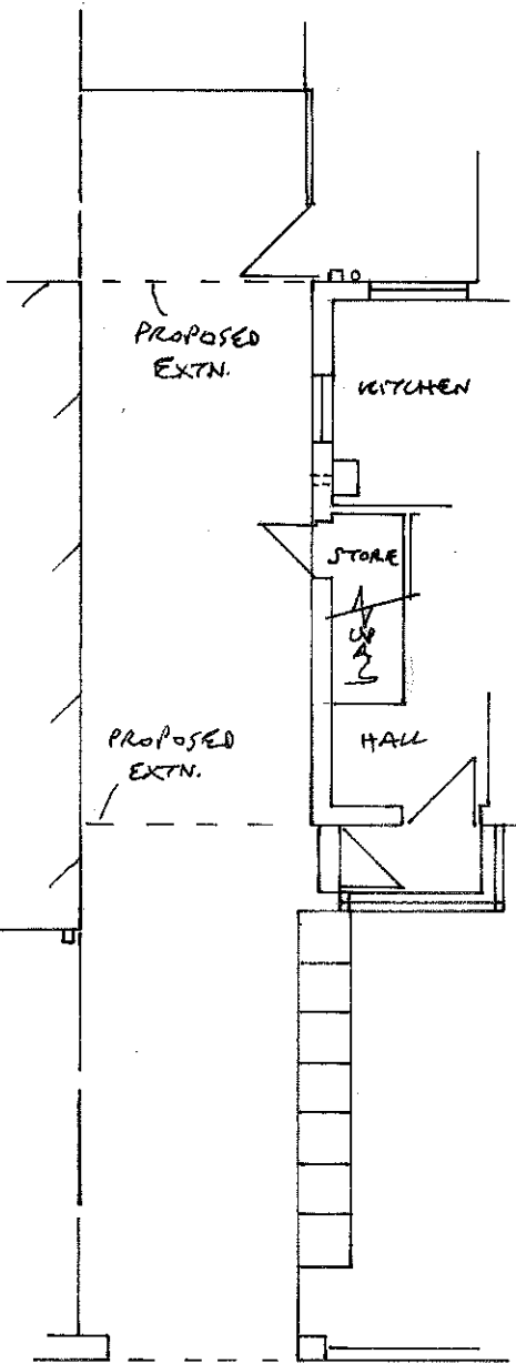
EXISTING PLAN 1:100
