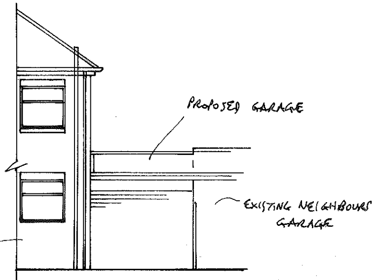
EXISTING/PROPOSED REAR 1:100
